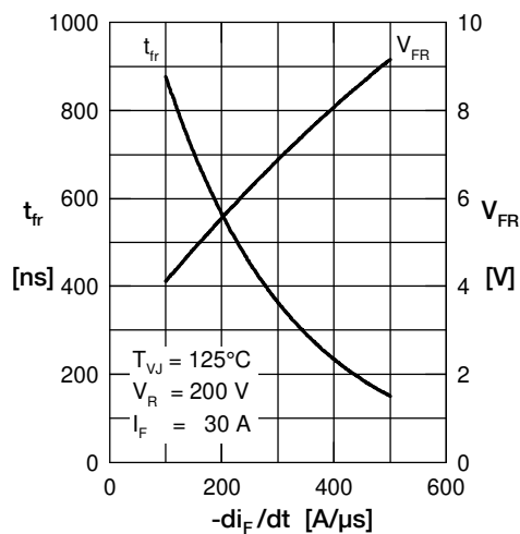
Fig. 6 Typ. forward recov. voltage V_{FR} & recovery time t_{fr} vs. di_F/dt
