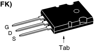
TO-264 (IXFK)
