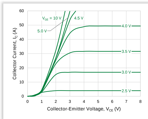
Figure 5. Output Characteristics ( T_J = 25\text{ }^{\circ}\text{C} )
