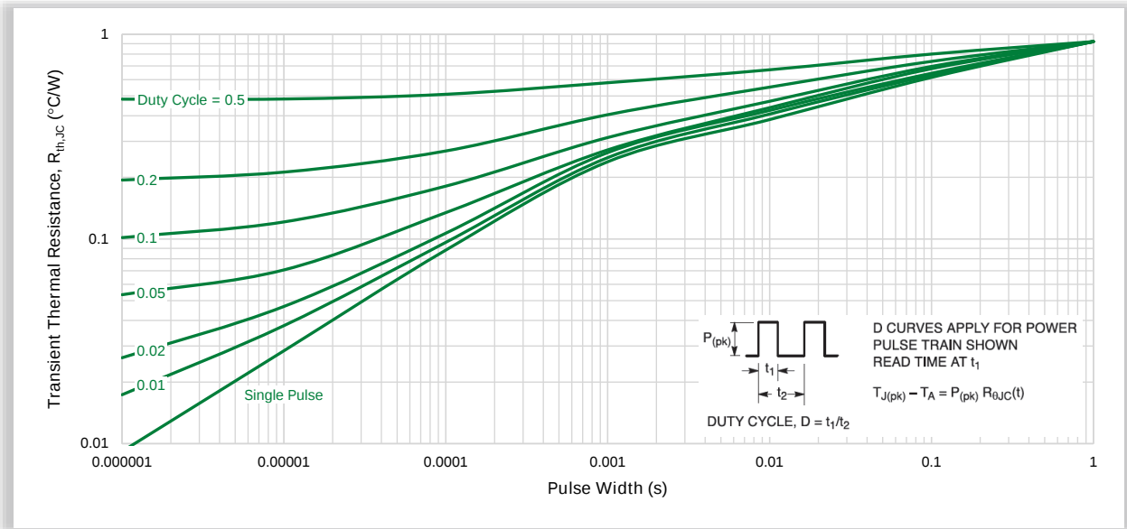
Figure 13. Best Case Transient Thermal Resistance
