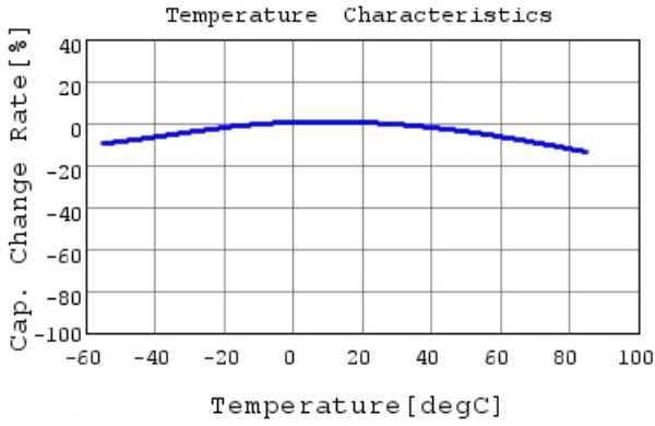
GRM219R61C226ME15 C-Temp. capchange, DC0.0V,
