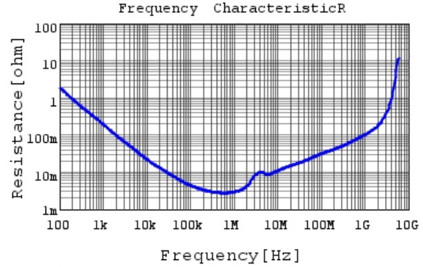
GRM219R61C226ME15 R DCOV, 25degC
