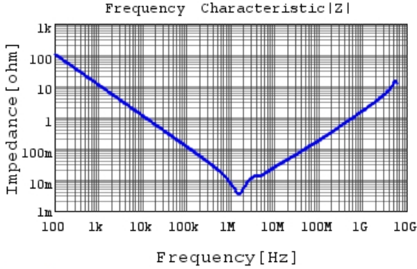
GRM219R61C226ME15 |Z| DCOV, 25degC
