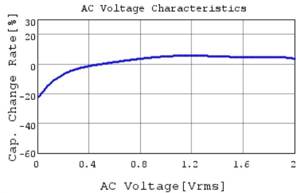
GRM219R61C226ME15 C-AC Voltage capchange, Dc
