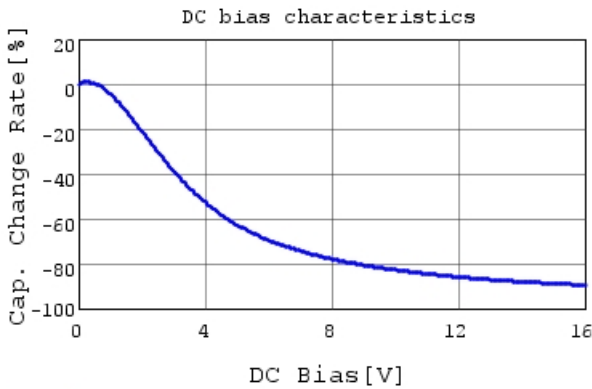
GRM219R61C226ME15 C-DC bias capchange, 25.0c
