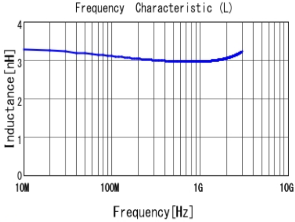
■ LQP03TN3N0BZ2 L
