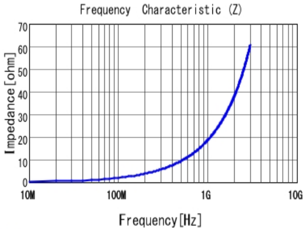
■ LQP03TN3N0BZ2 |Z|
