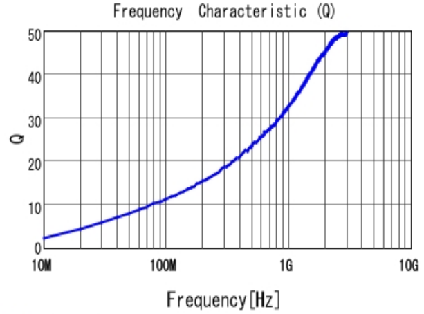
■ LQP03TN3N0BZ2 Q
