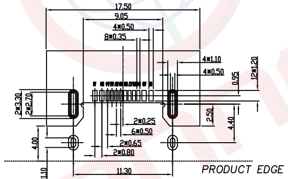
RECOMMENDED PCB LAYOUT(TOP VIEW) THICKNESS 0.8±0.10MM; DEFAULT TOLERANCE: ±0.05
