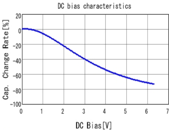
■ GRM155R70J105KA12 C-DC bias capchange, 25.0degC, AC1V
