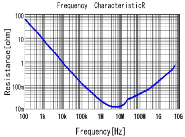
■ GRM155R70J105KA12 R DCOV, 25degC
