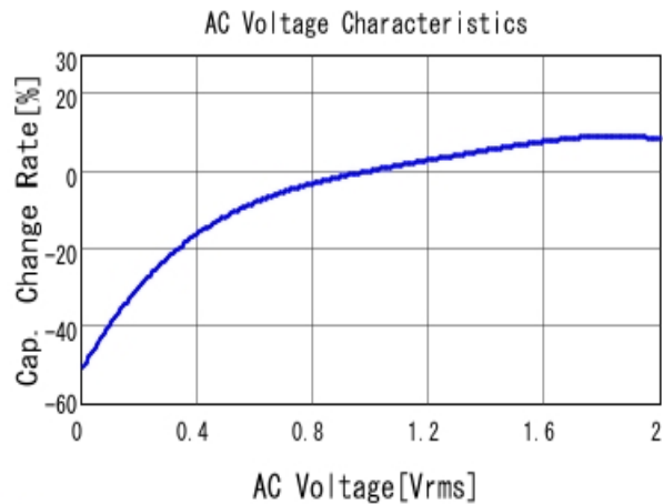
■ GRM155R70J105KA12 C-AC Voltage capchange, DCOV, 25.0d
