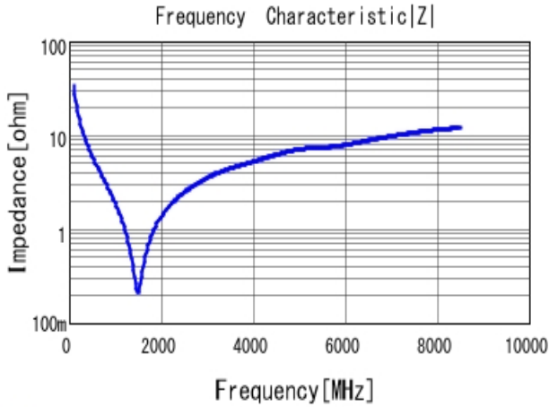
■ GRM0335C1H470JA01 |Z| DC0V, 25degC
