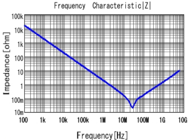
■ GRM155R71C104KA88 |Z| DC0V, 25degC
