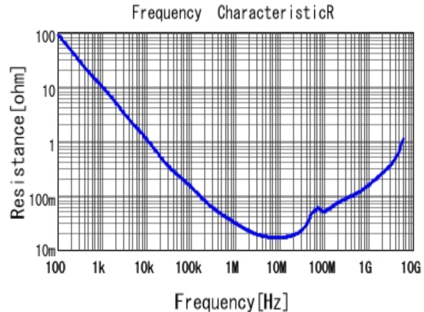
■ GRM155R71C104KA88 R DC0V, 25degC
