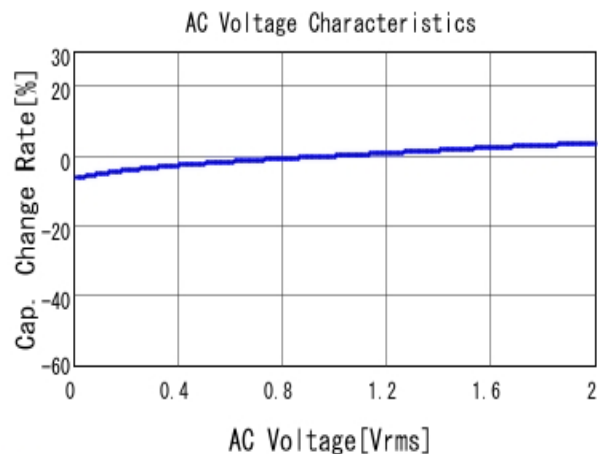
■ GRM155R71C104KA88 C-AC Voltage capchange, DC0V, 25.0d
