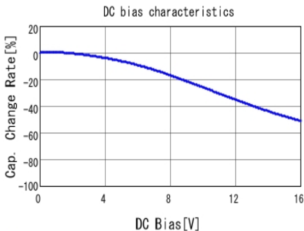
■ GRM155R71C104KA88 C-DC bias capchange, 25.0degC, AC1.
