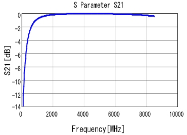
■ GRM1555C1H3R3BA01 S21 DCOV, 25degC
