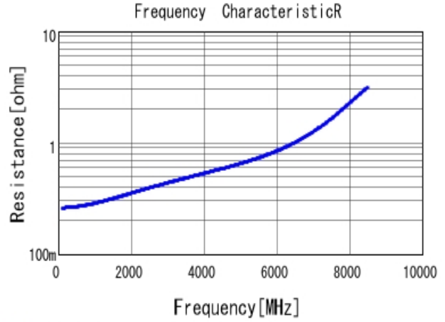
■ GRM1555C1H3R3BA01 R DC0V, 25degC
