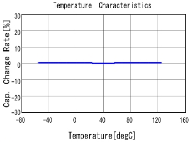
■ GRM1555C1H3R3BA01 C-Temp. capchange, DCOV, AC1Vrms
