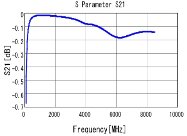
■ GRM0335C1H390JA01 S21 DCOV, 25degC
