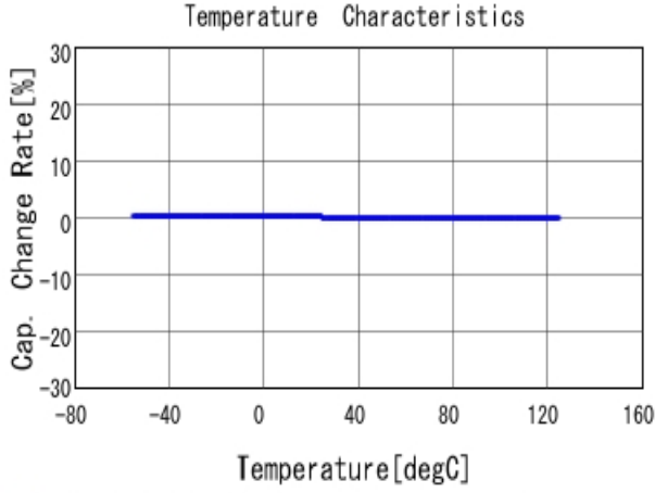
■ GRM0335C1H390JA01 C-Temp. capchange, DCOV, AC1Vrms
