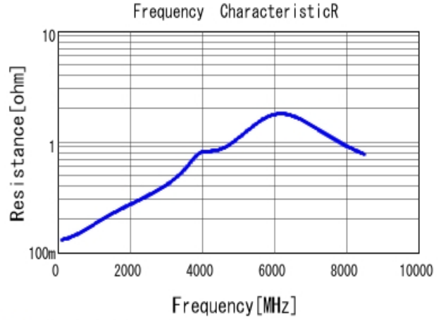
■ GRM0335C1H390JA01 R DC0V, 25degC
