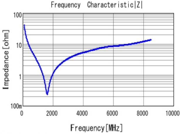
■ GRM0335C1H390JA01 |Z| DC0V, 25degC
