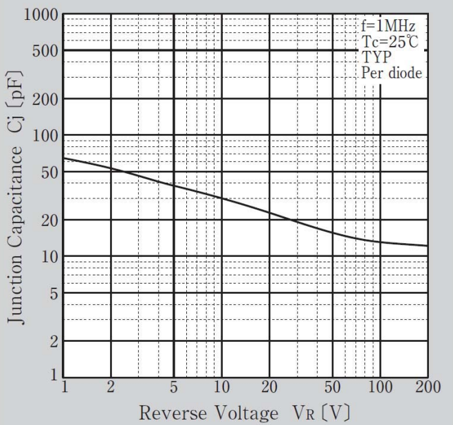
Junction Capacitance
