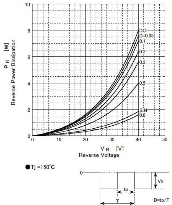
SG15SC4M Reverse Power Dissipation
