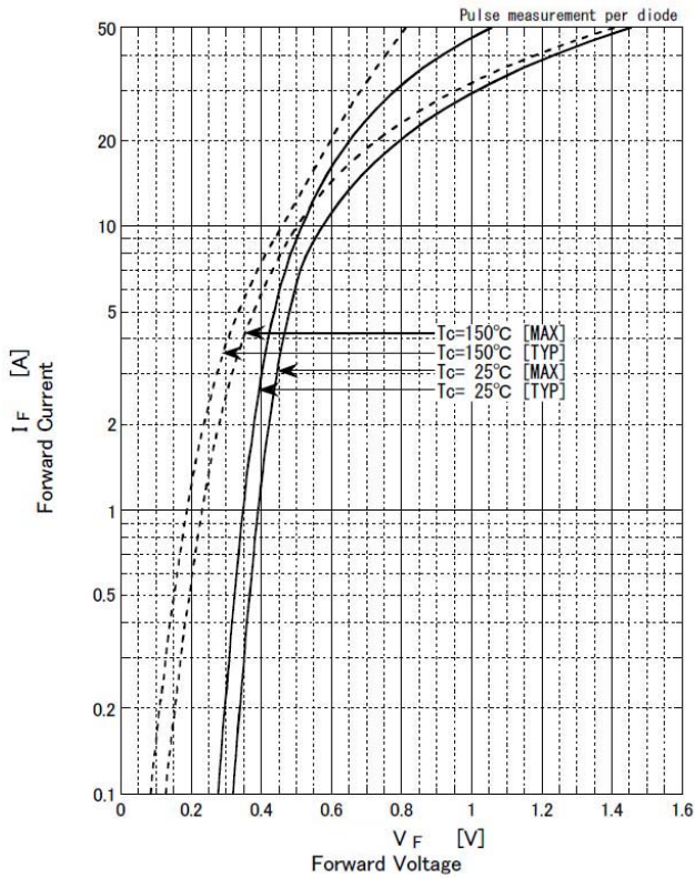
SG15SC4M Forward Voltage
