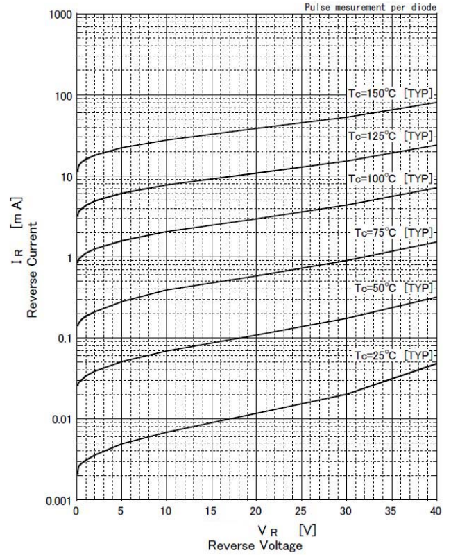
SG15SC4M Reverse Current
