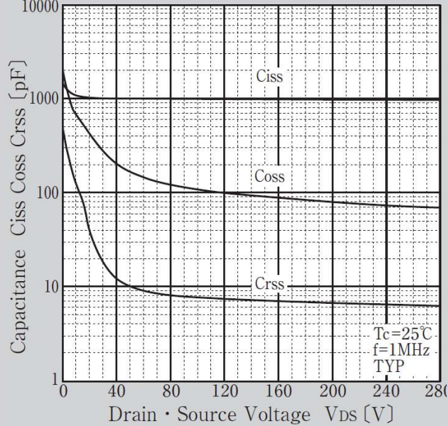
Capacitance Characteristics
