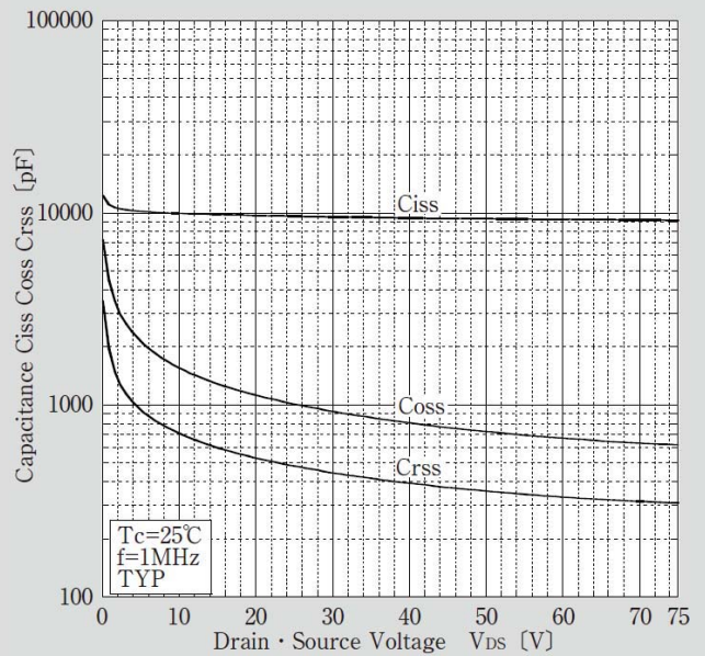
Capacitance Characteristics
