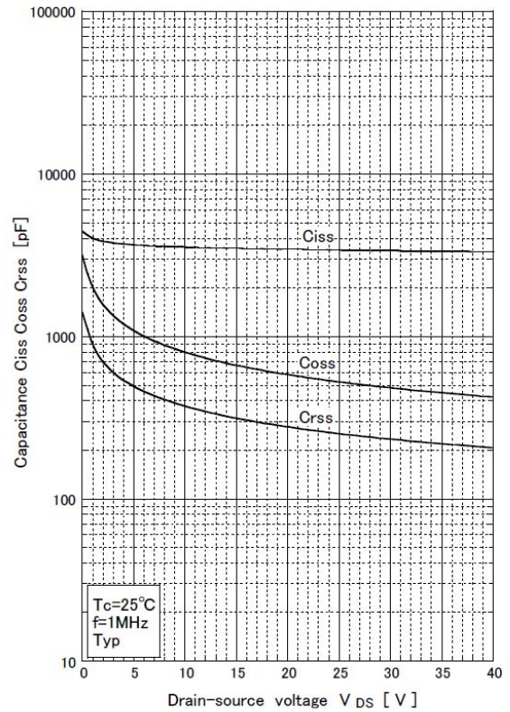
Capacitance characteristics
