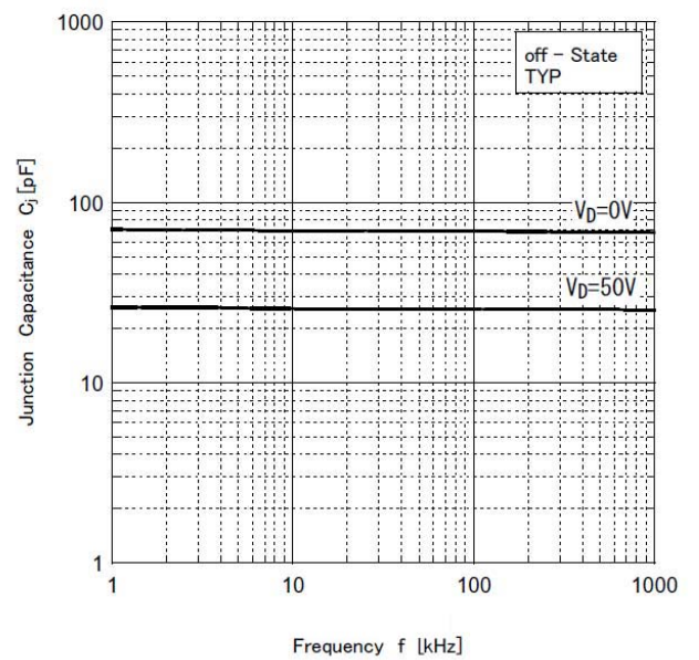
Junction Capacitance
