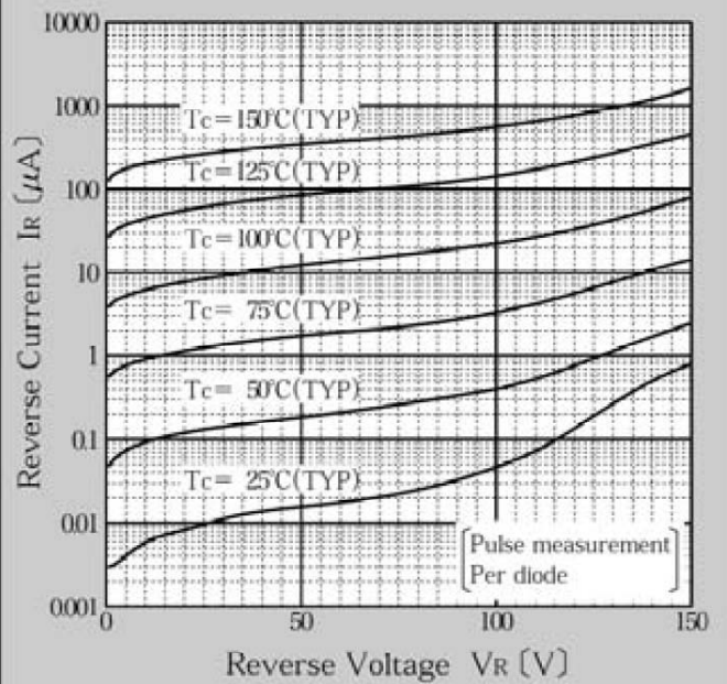
Reverse Current
