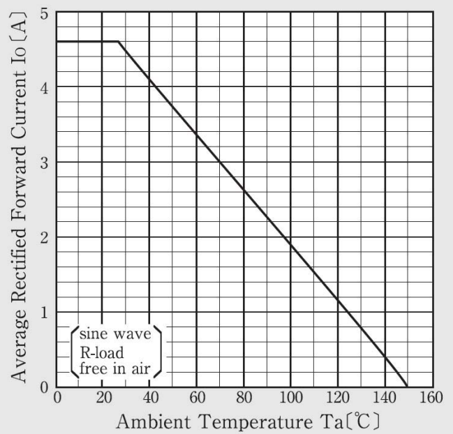
Derating Curve
