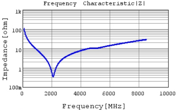
GRM1555C1E150JA01 |Z| DCOV, 25degC
