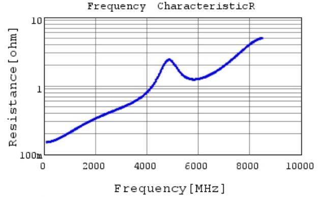
GRM1555C1E150JA01 R DCOV, 25degC
