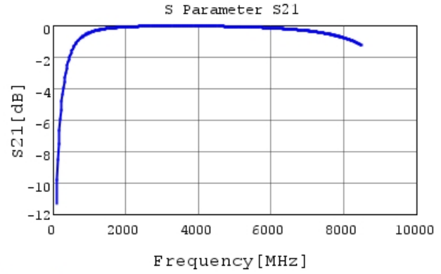
GRM1555C1H4R5BA01 S21 DCOV, 25degC
