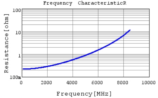
GRM1555C1H4R5BA01 R DC0V, 25degC
