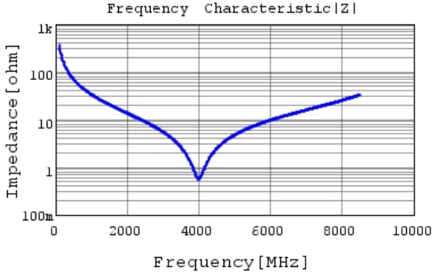
GRM1555C1H4R5BA01 |Z| DC0V, 25degC
