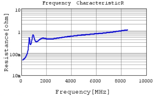
GCM1555C1H821FA16 R DCOV, 25degC
