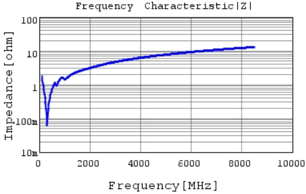
GCM1555C1H821FA16 |Z| DCOV, 25degC
