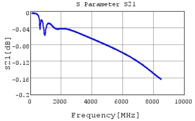
GCM1555C1H821FA16 S21 DCOV, 25degC
