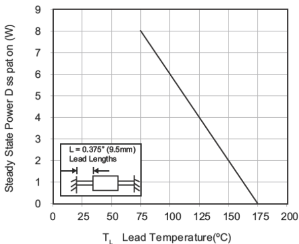
Figure 5 - Steady State Power Derating Curve
