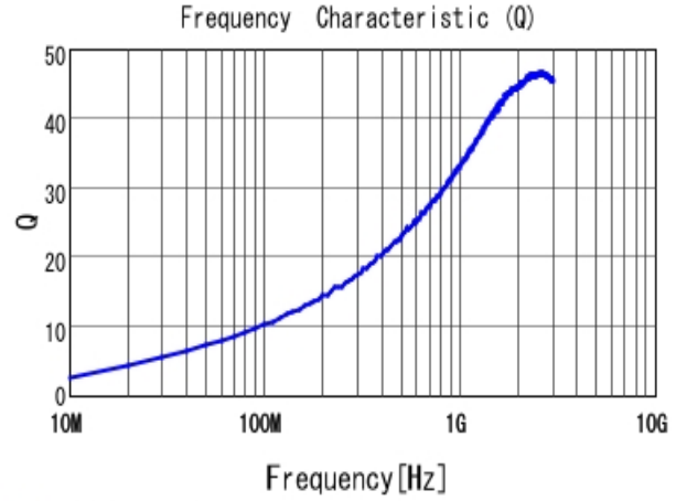
■ LQG15HS2N2C02 Q
