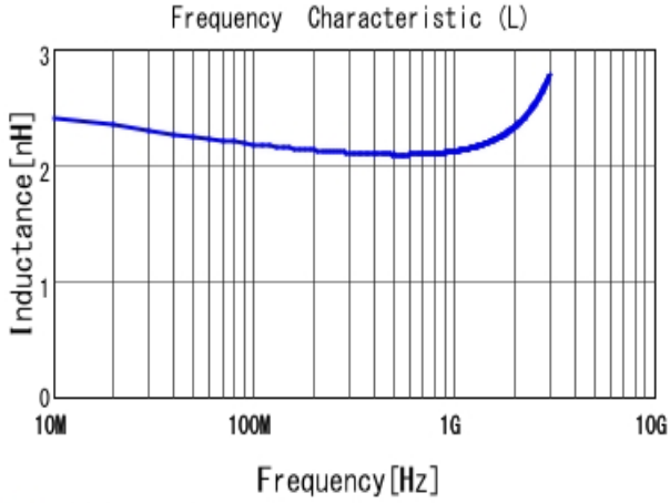
■ LQG15HS2N2C02 L
