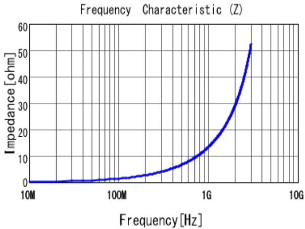
■ LQG15HS2N2C02 |Z|
