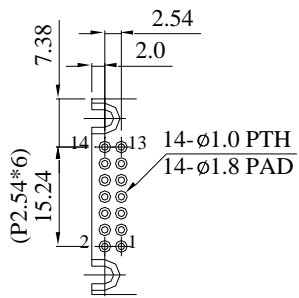
PIN DETAIL
