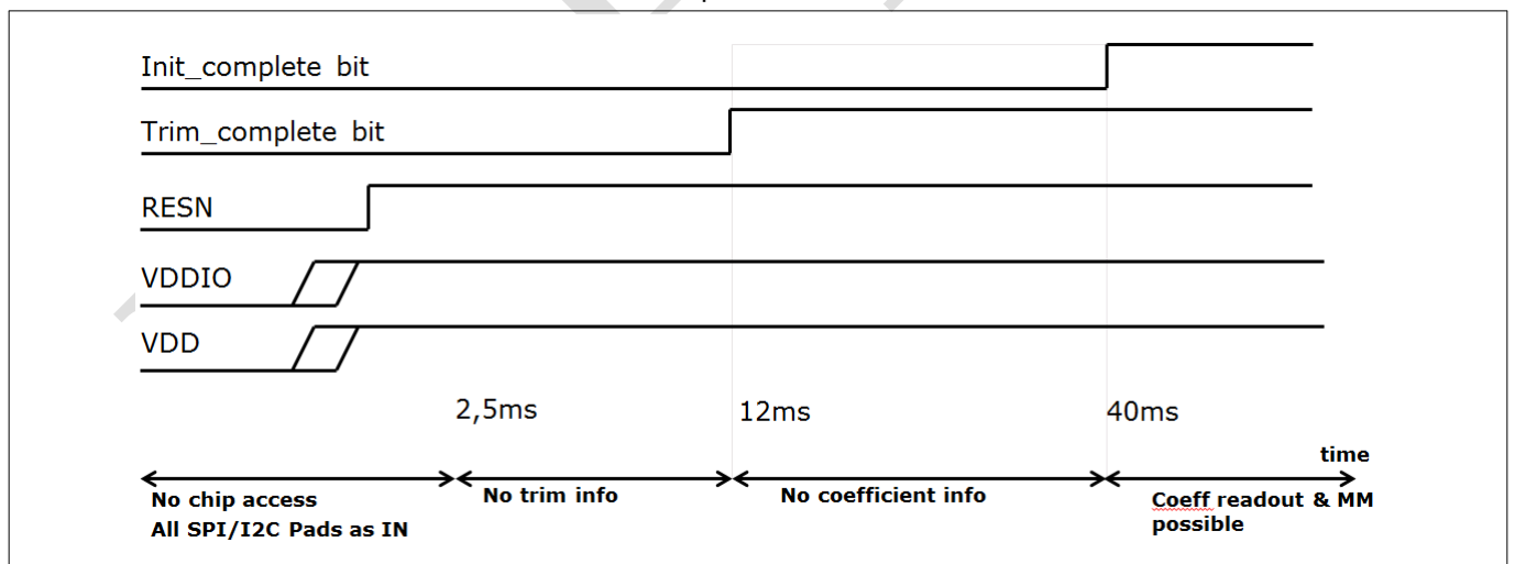
Figure 8: Start-up sequence
