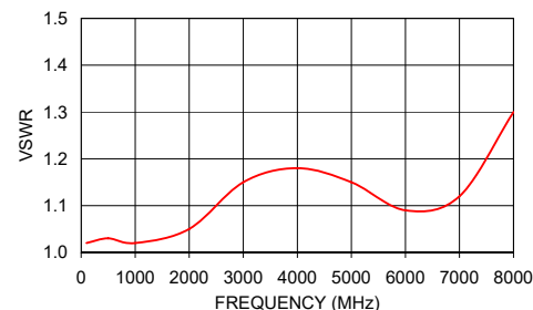
GAT-1+ VSWR
