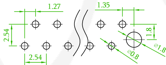
Recommended PCB Layout (PCB TOLERANCE ±0.05)
