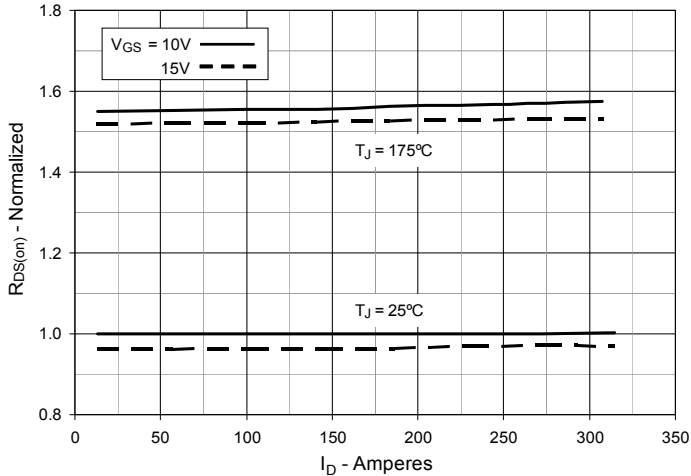
Fig. 5. Normalized R_{DS(on)} to I_D = 100A vs. Drain Current
