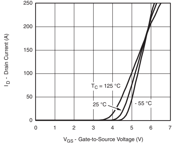
T_C = 125\text{ }^\circ\text{C} 25\text{ }^\circ\text{C} -55\text{ }^\circ\text{C} V_{GS} - Gate-to-Source Voltage (V) Transfer Characteristics
