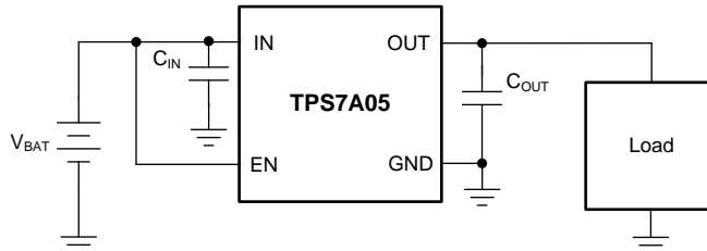
Figure 53. Operation From the Battery Input Supply
