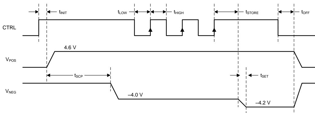
Figure 7. Programming V_{NEG} Using the CTRL Pin
