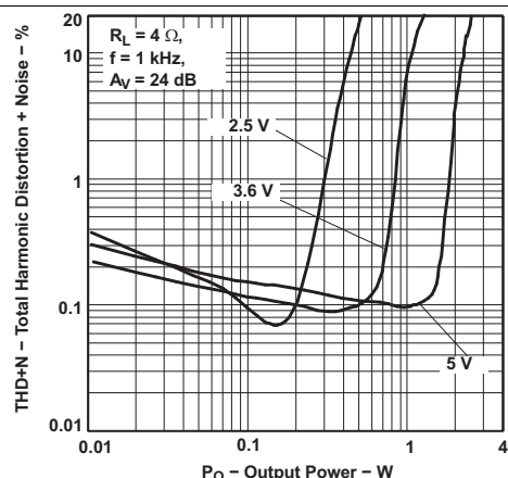
Figure 3. Total Harmonic Distortion vs Output Power
