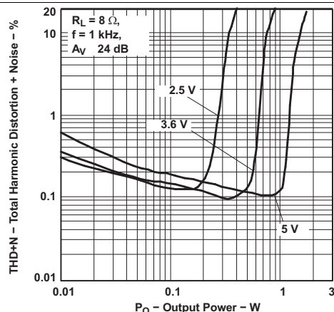
Figure 1. Total Harmonic Distortion vs Output Power
