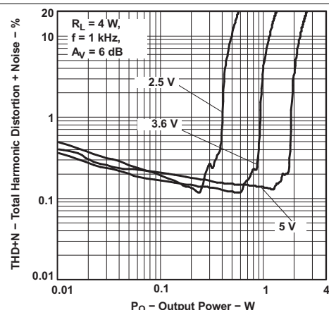
Figure 4. Total Harmonic Distortion vs Output Power
