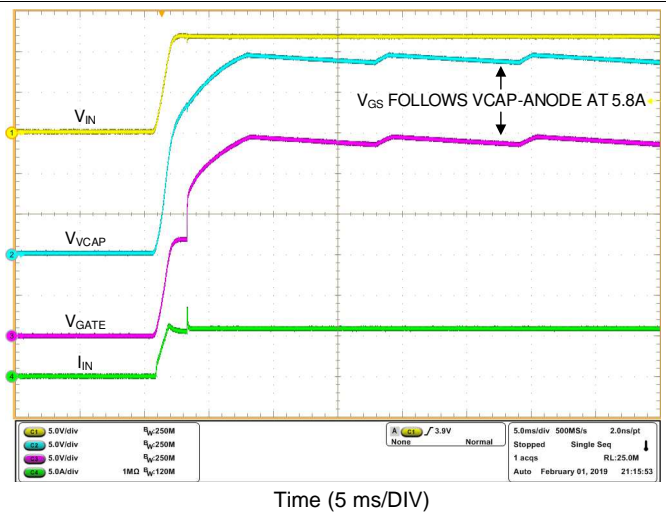
Figure 27. VCAP during startup at 5.8-A Load
