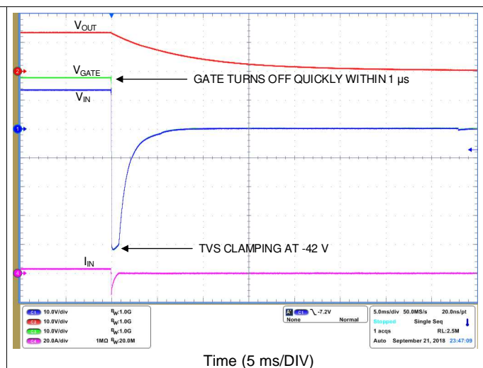
Figure 23. Response to ISO 7637-2 Pulse 1
