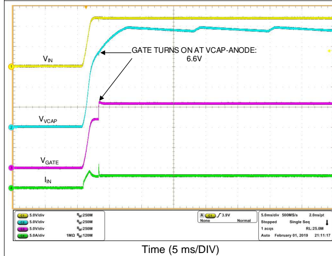
Figure 26. VCAP during startup at 3-A Load
