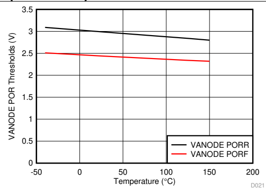
Figure 14. VANODE POR Threshold vs Temperature
