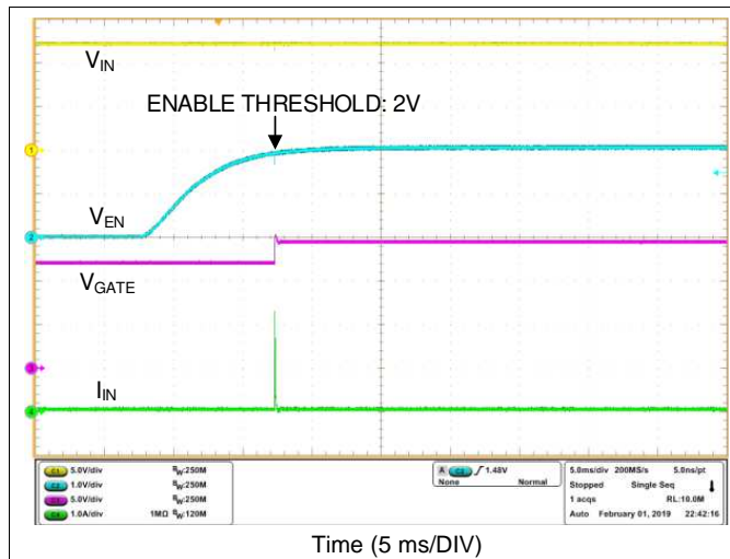
Figure 28. Enable Threshold
