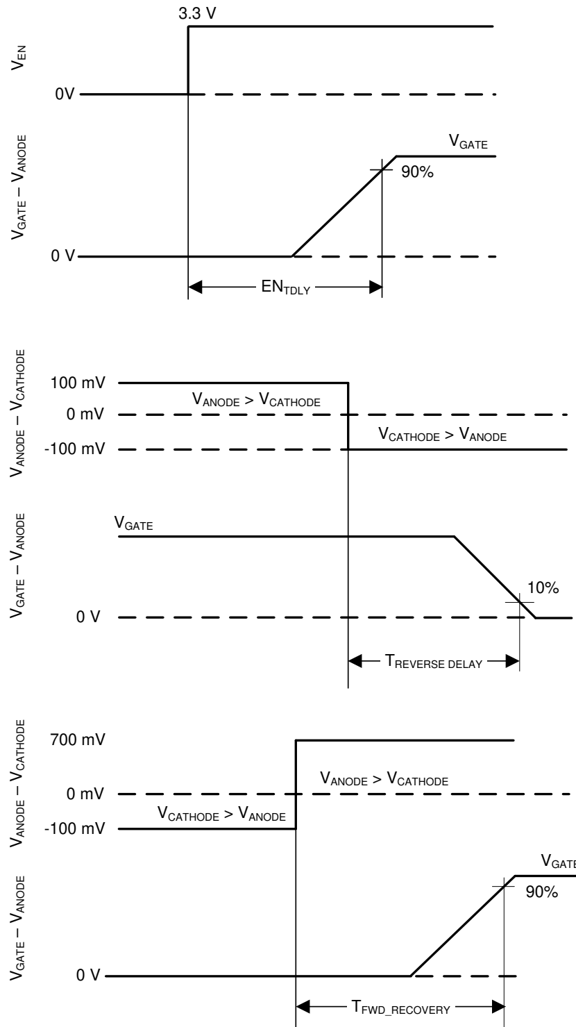
Figure 16. Timing Waveforms
