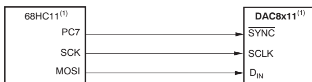
Figure 83. DAC8X11 to 68HC11 Interface
