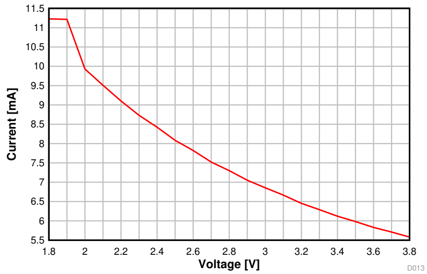
Figure 5-7. RX Current vs. Supply Voltage (VDD5) (BLE 1 Mbps, 2.44 GHz)
