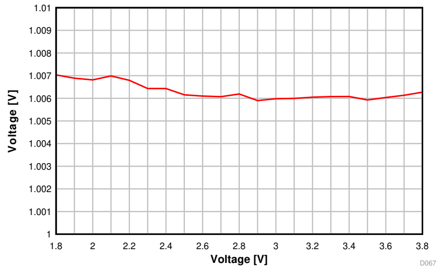
Figure 5-25. ADC Accuracy vs. Supply Voltage (VDDS)
