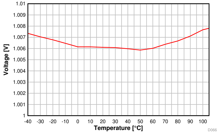
Figure 5-24. ADC Accuracy vs. Temperature
