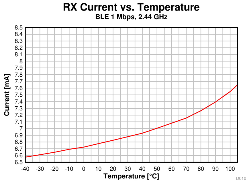
Figure 5-6. RX Current vs. Temperature (BLE 1 Mbps, 2.44 GHz)
