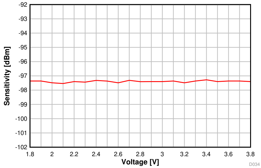
Figure 5-12. Sensitivity vs. Supply Voltage (VDD5) (BLE 1 Mbps, 2.44 GHz)
