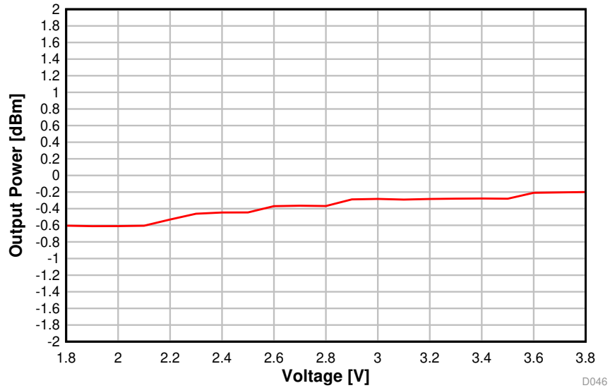
Figure 5-16. Output Power vs. Supply Voltage (VDDS) (BLE 1 Mbps, 2.44 GHz)
