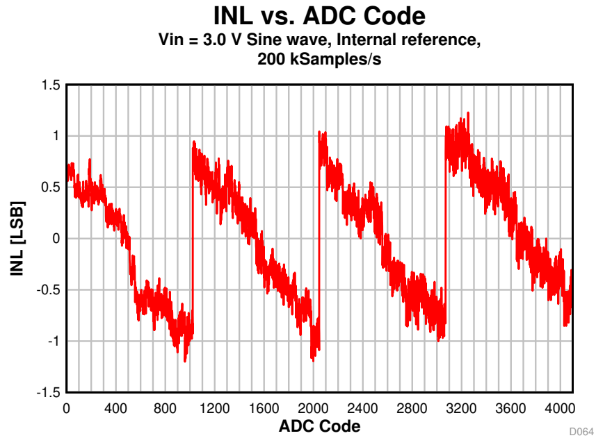
Figure 5-22. INL vs. ADC Code
