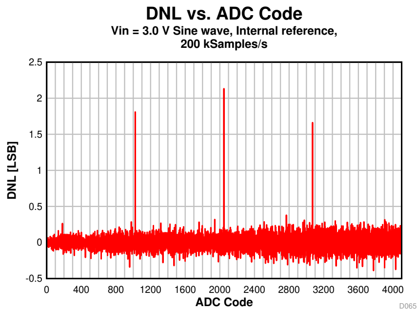
Figure 5-23. DNL vs. ADC Code
