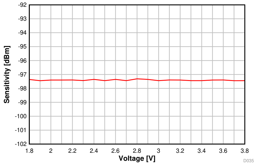
Figure 5-13. Sensitivity vs. Supply Voltage (VDD5) (BLE 1 Mbps, 2.44 GHz, DCDC Off)
