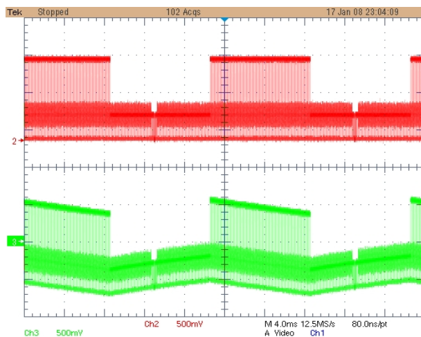
Figure 14. C_{sag} = 22\ \mu\text{F} , C_{out} = 47\ \mu\text{F} (Top : Input, Bottom : Output)
