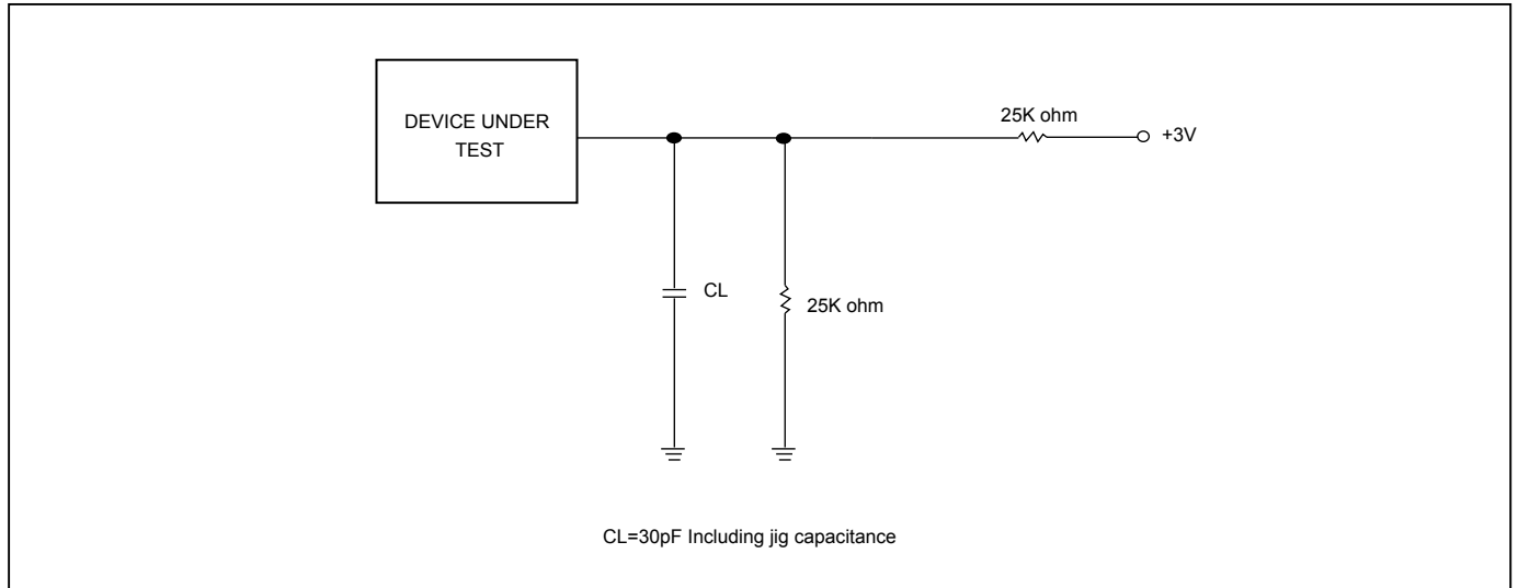
Figure 127. OUTPUT LOADING
