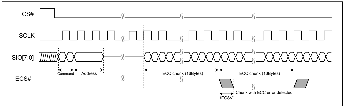
Figure 117. ECS# Timing
