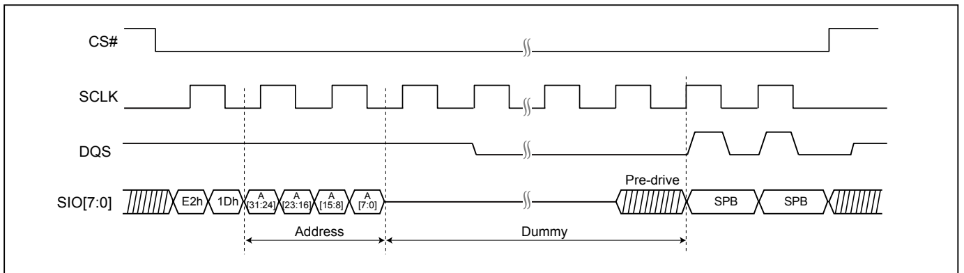
Figure 85. Read SPB Status (RDSPB) Sequence (DTR-OPI Mode)
