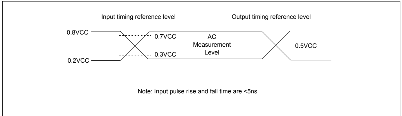
Figure 126. INPUT TEST WAVEFORMS AND MEASUREMENT LEVEL
