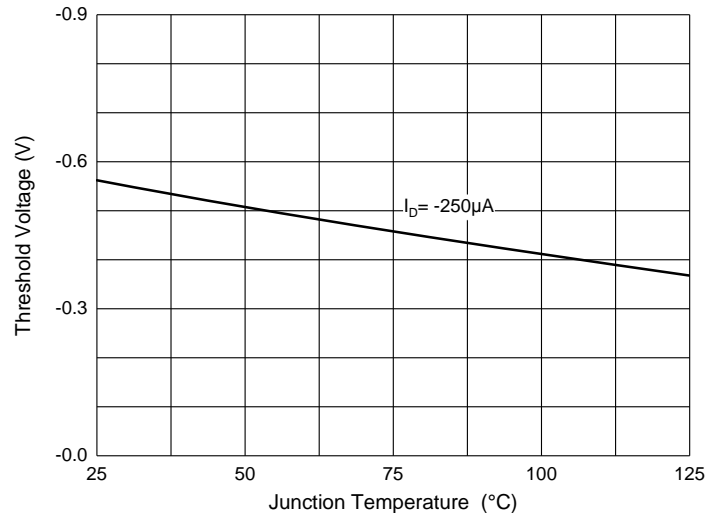
Fig. 6 - Threshold Voltage
