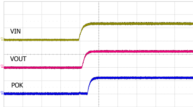
VIN : 2.0V/div, VOUT : 1.0V/div, POK : 2.0V/div, Time : 1ms/div Start Up @ I out =1A
