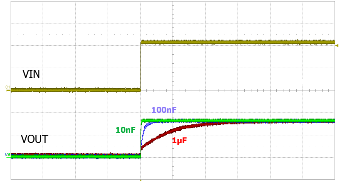
VIN : 2.0V/div, VOUT : 2.0V/div, Time : 50ms/div Start Up @ I out =10mA
