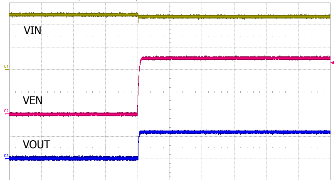
VIN : 1.0V/div, VEN : 1.0V/div, VOUT : 1.0V/div, Time : 5ms/div Start Up by External VEN @ I out =1A
