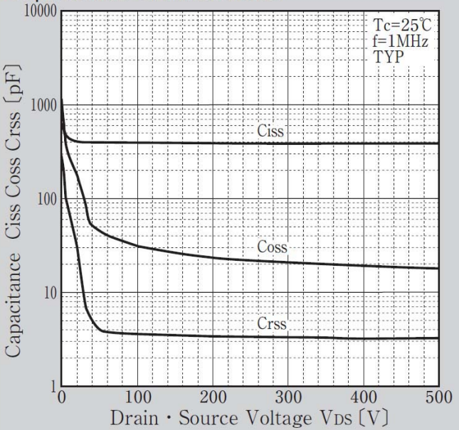
Capacitance Characteristics
