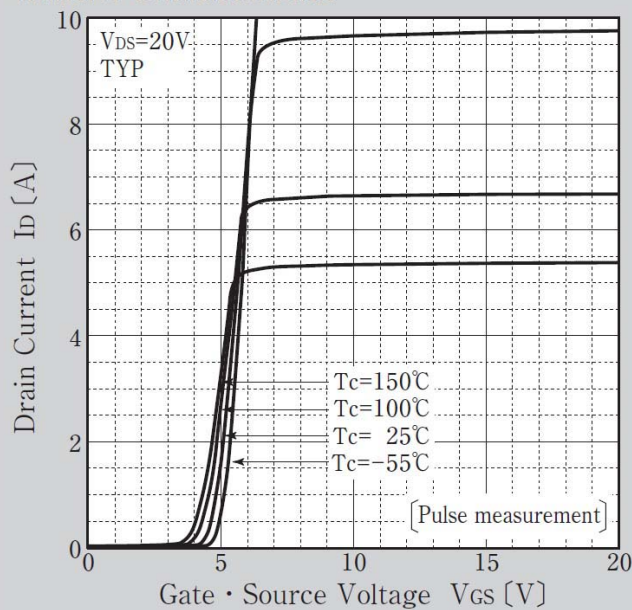
Transfer Characteristics
