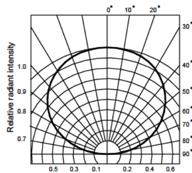
Fig.6 Radiation diagram
