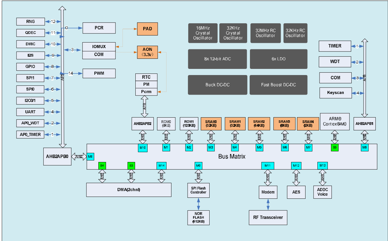
Figure 1: CMT4501 block diagram
