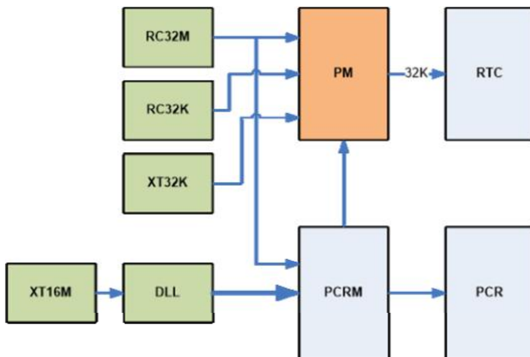
Figure 10: Clock management
