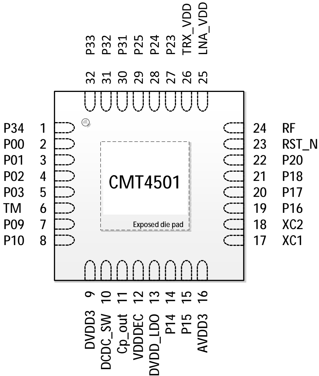
Figure 3: Pin assignment - CMT4501 QFN32 package
