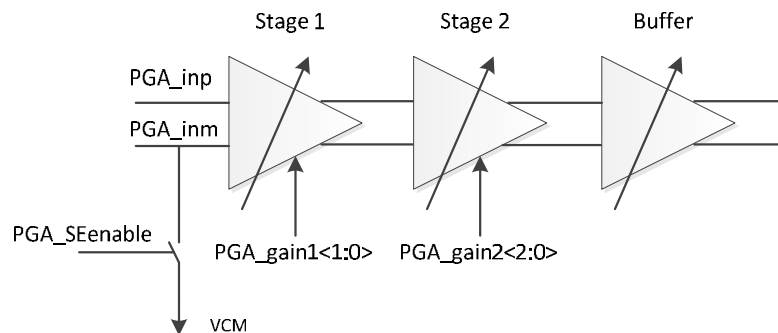
Figure 13: PGA path
