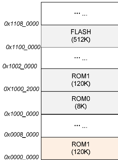
Figure 5: CMT4501 boot mode
