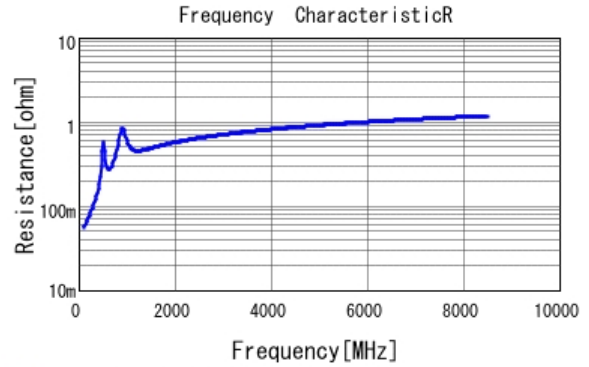
■ GRM1885C1H681JA01 R DCOV, 25degC
