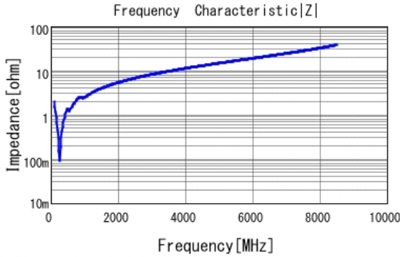
■ GRM1885C1H681JA01 |Z| DCOV, 25degC
