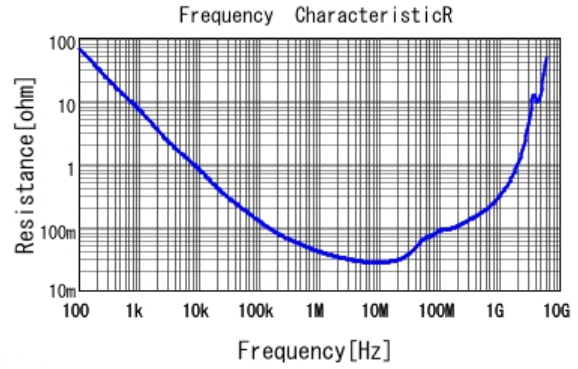
■ GRM319R72A104KA01 R DCOV, 25degC
