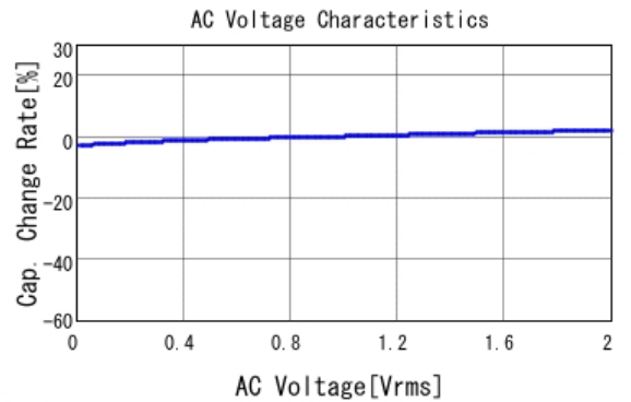
■ GRM319R72A104KA01 C-AC Voltage capchange, DCOV, 25.0d
