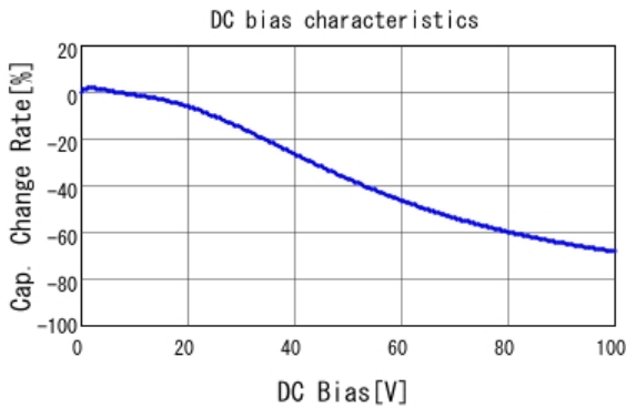
■ GRM319R72A104KA01 C-DC bias capchange, 25.0degC, AC1.
