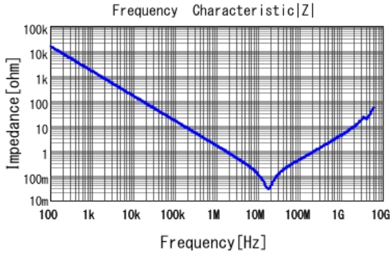
■ GRM319R72A104KA01 |Z| DCOV, 25degC
