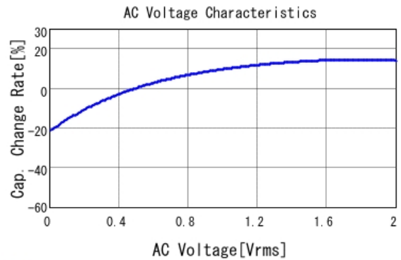
■ GRM21BR61C106KE15 C-AC Voltage capchange, DCOV, 25.0d
