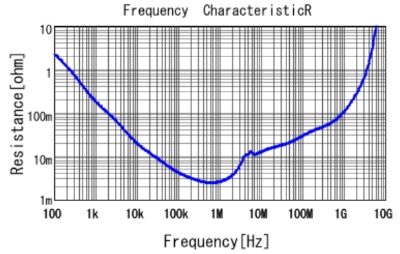
■ GRM21BR61C106KE15 R DCOV, 25degC
