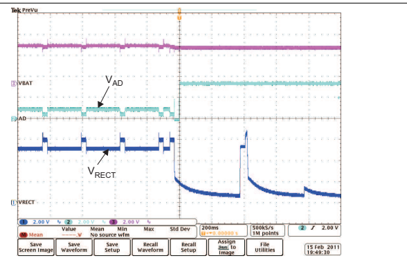
Figure 16. On-the-Go Enabled ( V_{OTG} = 3.5\text{ V} ) (3)
