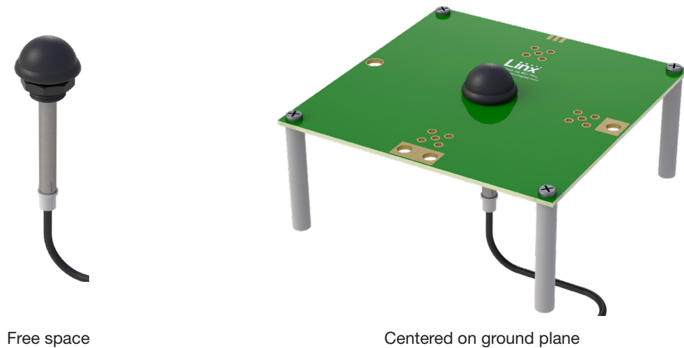
Figure 3. ANT-DB1-WRT-ccc Test Orientations
