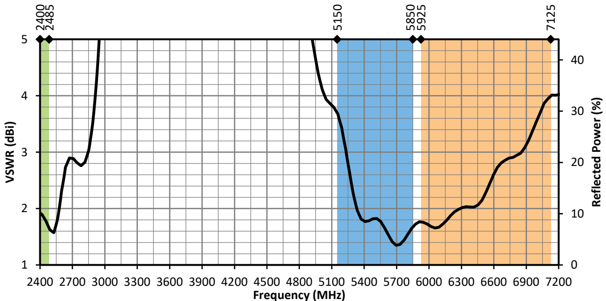
Figure 5. ANT-DB1-WRT-ccc VSWR, Freespace
