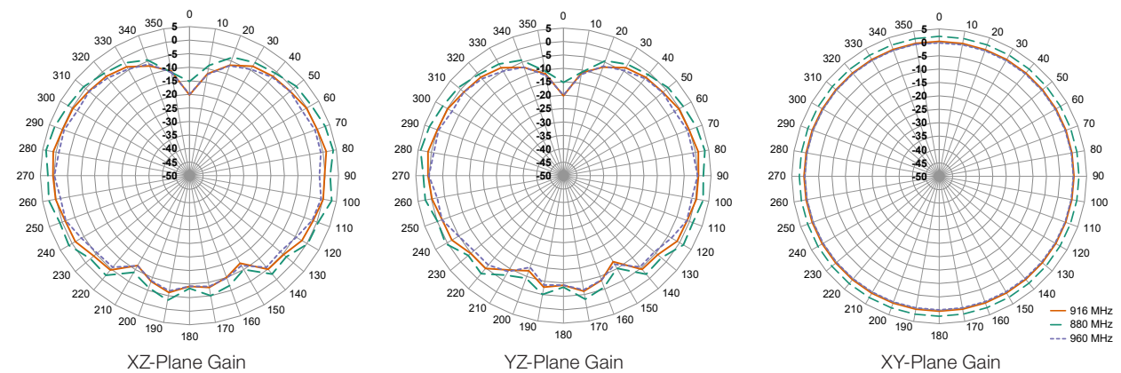
Figure9. Radiation Patterns for CW LTE Band 8 Antenna
