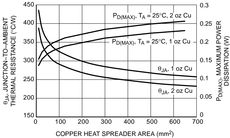
Figure 46. θ JA vs. Copper Area (TSOP-5)
